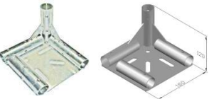
GP – B85 [SUPPORT WITH STOP FOR 85MM ROLLER TRACK]
