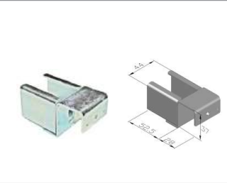
GP – F [ STANDARD TRACK SUPPORT - Y STYLE ]
