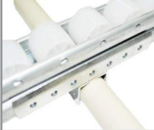
GP – C1L [ ROLLER SPLICE WITH CENTRE SUPPORT ]
