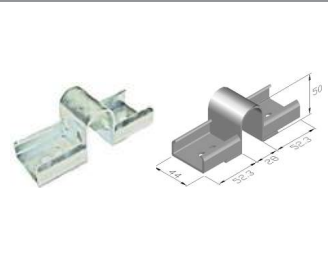
GP – HR [ ROLLER TO ROLLER SUPPORT ]
