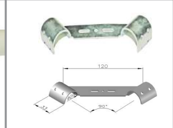
CM – A [ BOARD CORNER SUPPORT A ]
