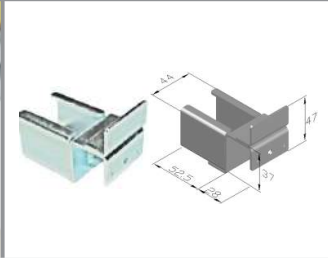
GP – G [ STANDARD TRACK SUPPORT-WITH TAB STOP ]
