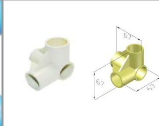
GAP – 2B [ 3 WAY HOLL PLASTIC JOINT ]
