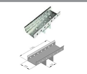
GP – C1 [ ROLLER SPLICE WITH CENTRE SUPPORT ]
