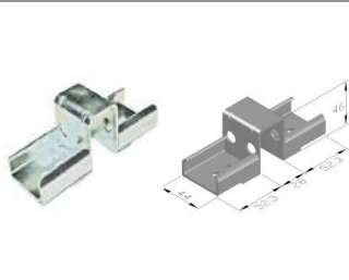
GP – H [ ROLLER TO ROLLER SUPPORT ]
