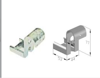
GP – D [ ROLLER SUPPORT WITH LARGE STOP ]
