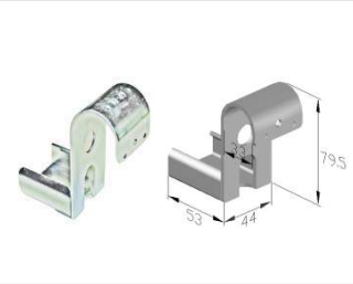
GP – DL [ ROLLER SUPPORT WITH LARGE STOP ]
