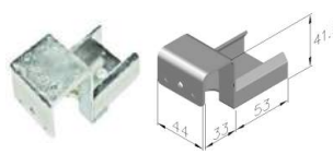
GP – B [ ROLLER SUPPORT WITH STOP ]
