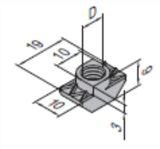
T Nut-10-M4 T Nut-10-M5 T Nut-10-M6 T Nut-10-M8
