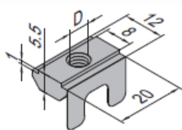
Subsequent Nut-8-M4 Subsequent Nut-8-M5 Subsequent Nut-8-M6
