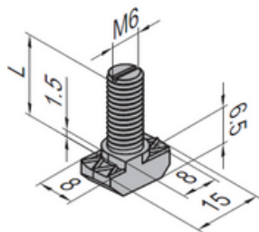
T Bolt-8-16 T Bolt-8-20 T Bolt-8-25
