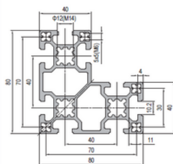
80x80 L 8 slots
