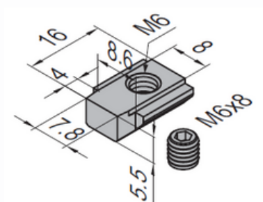
Anti-torsion Subsequent Nut-8
