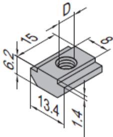
Pre-set Nut-8-M4 Pre-set Nut-8-M5 Pre-set Nut-8-M6 Pre-set Nut Sleeve-8
