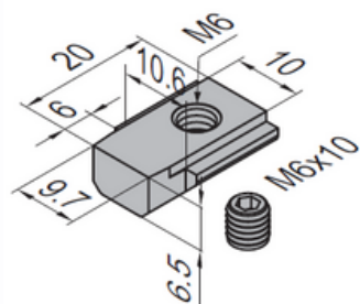
Anti-torsion Subsequent Nut-10
