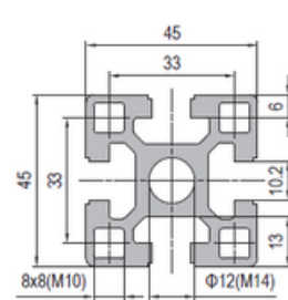
45x45 4 slots Heavy
