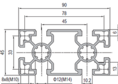
45x90 6 slots light
