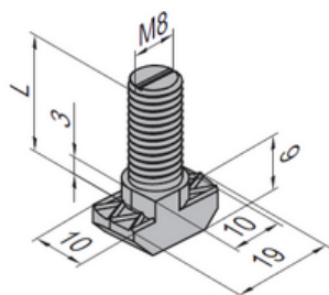
T Bolt-10-20 T Bolt-10-25 T Bolt-10-30 T Bolt-10-35
